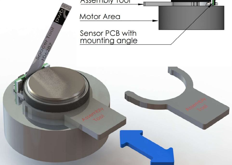
Spacer Tool for AS25 and AS50 Thickness 0,2mm
