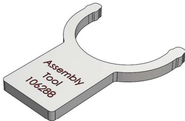
Art. Nr.: 106288: Assembly Tool for AS25 Thickness 5mm For the magnet wheels as press fit version with max. shaft diameter 20mm
