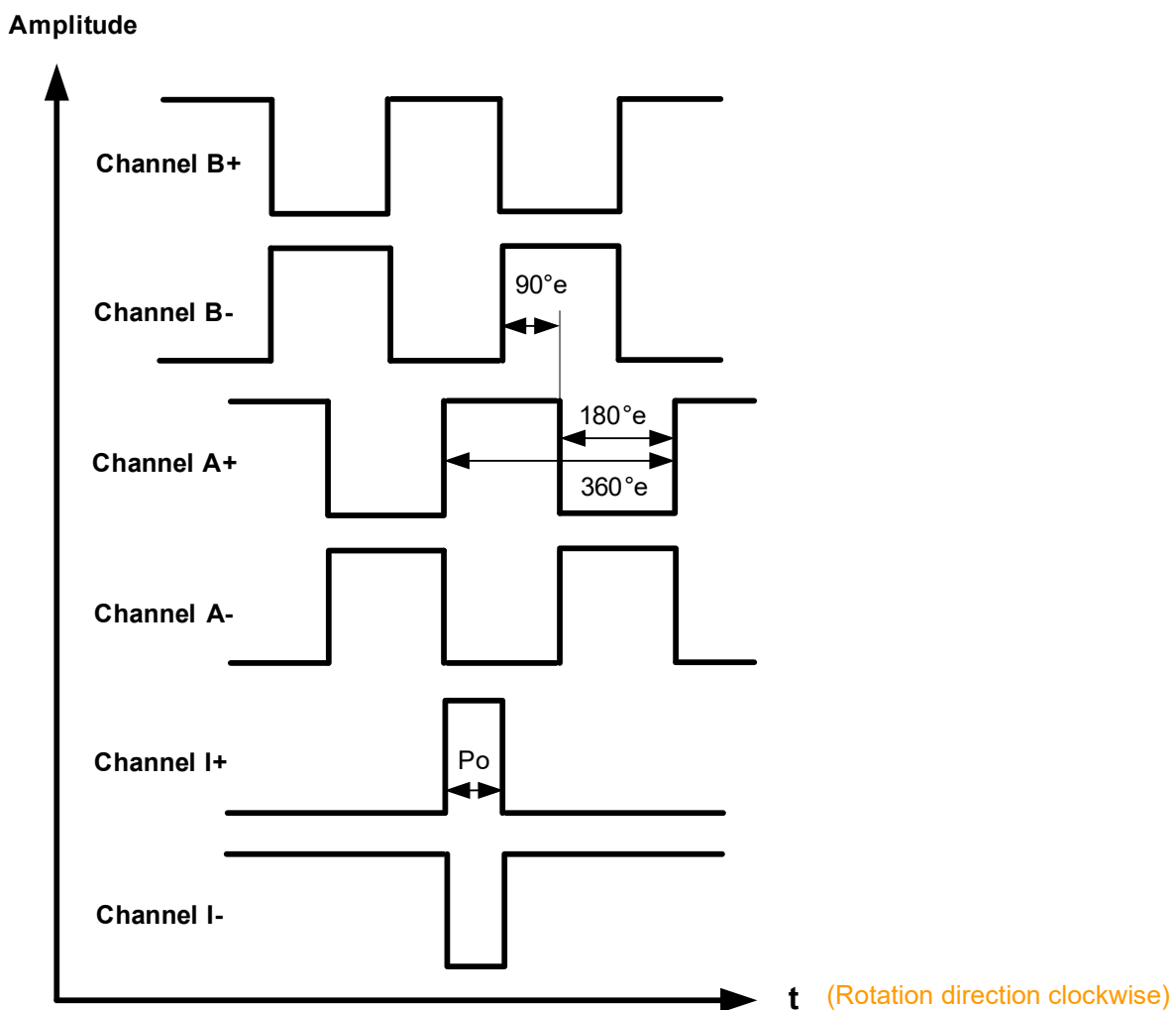
Figure: Incremental interface with differential signals
